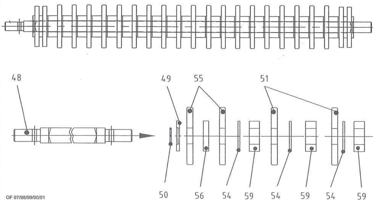
Grading roller 20mm
