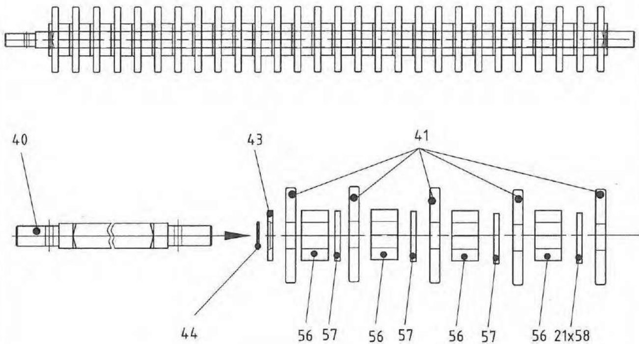
Kalibrierwelle LW30mm
