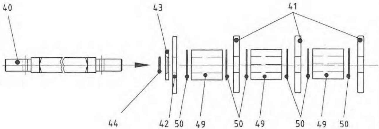
Kalibrierwelle LW40mm
